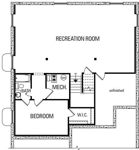
OPT. FINISHED BASEMENT 1277 SQ. FT
