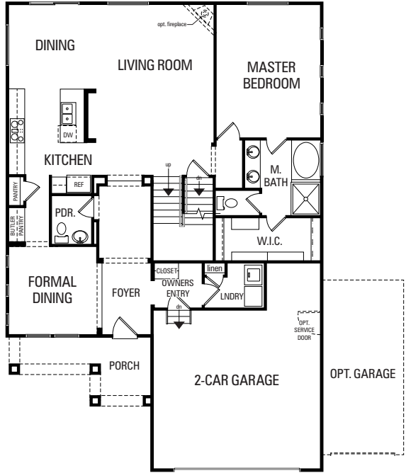
MAIN FLOOR 1546 SQ. FT
