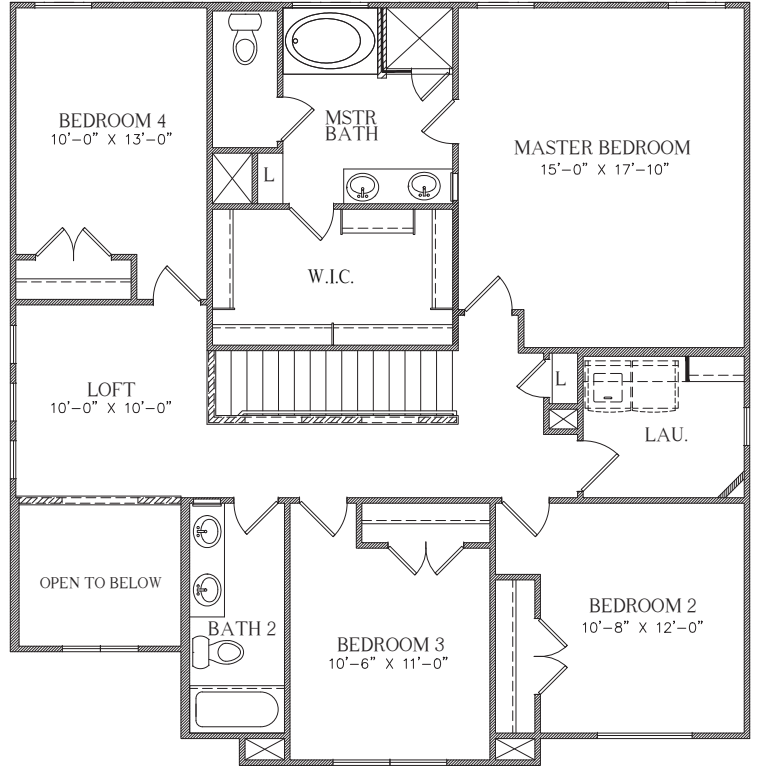
2453 SECOND FLOOR
