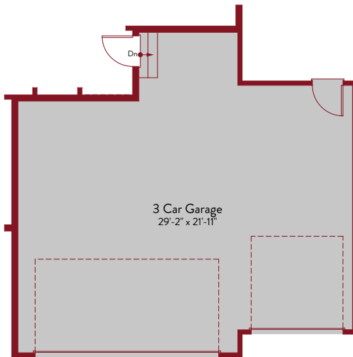
Opt. 3 Car Garage
