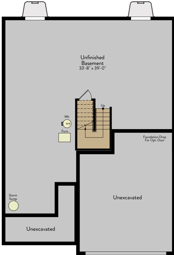
Opt. Unfinished Basement - 987 sq. ft.
