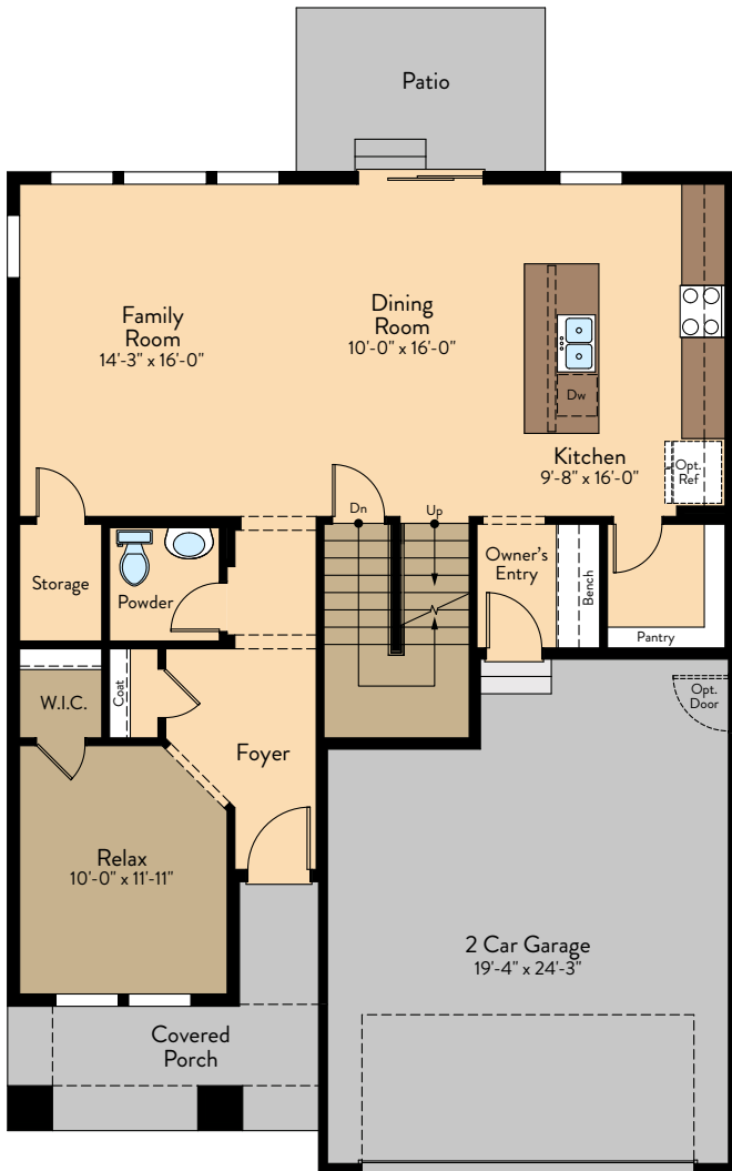
FIRST FLOOR - 1083 SQ. FT.
