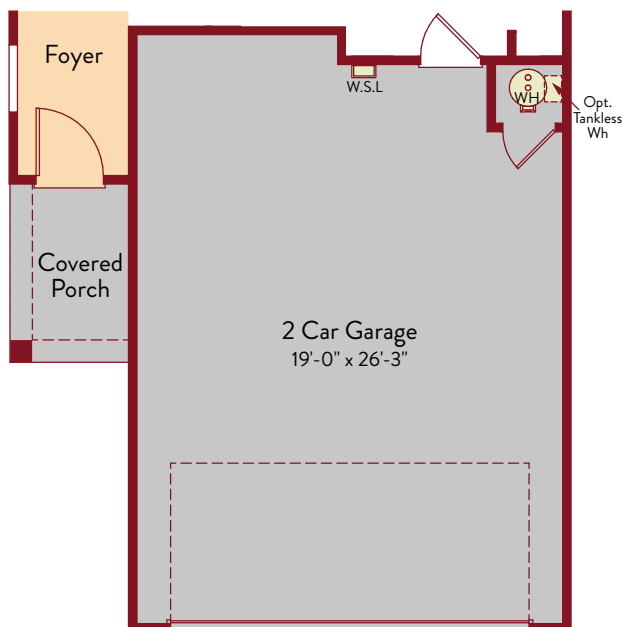
Opt. 4' Garage Extension
