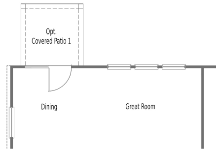
Optional Covered Patio 1 Partial Main Floor Plan
