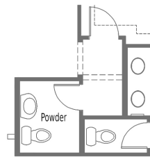
Optional Powder I.L.O. Storage Partial Main Floor Plan
