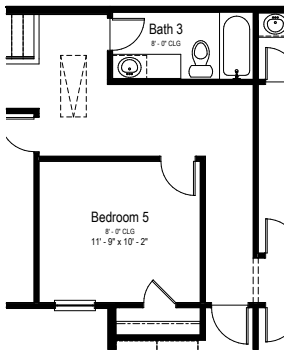
Opt. Bedroom 5 Partial Upper Floor Plan
