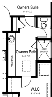
Opt. 42x60 Shower Partial Main Floor Plan
