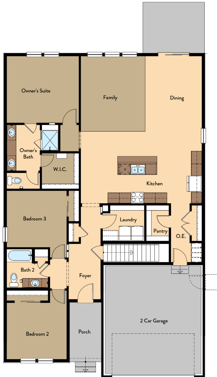
Main Level
