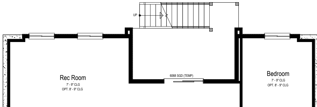
OPT DAYLIGHT BASEMENT PARTIAL BASEMENT PLAN
