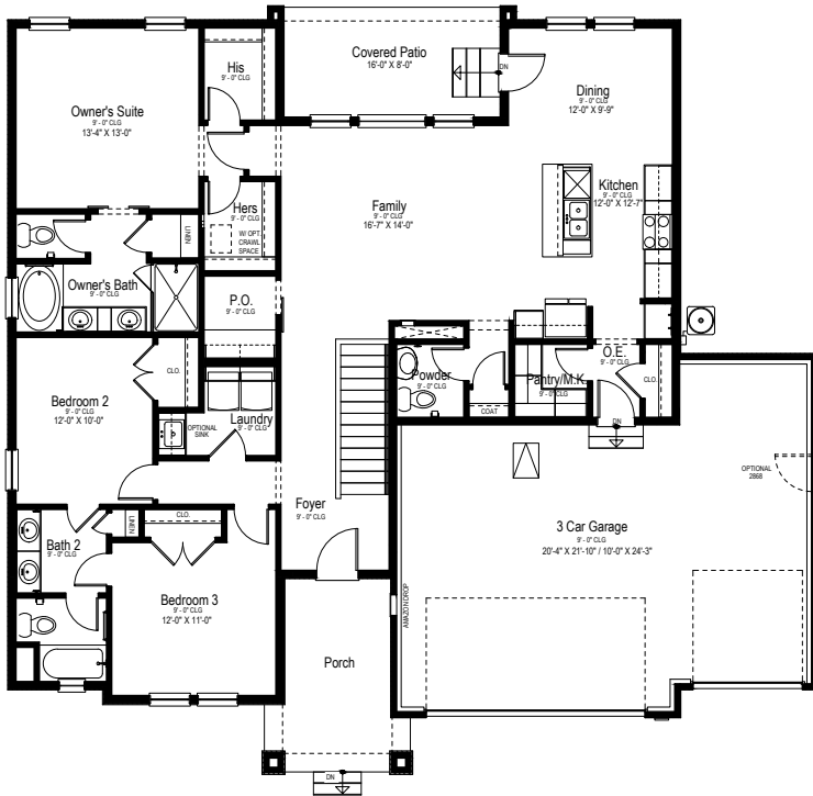
FIRST FLOOR - 3 CAR GARAGE (24')
