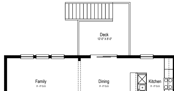
OPT WALKOUT BASEMENT PARTIAL MAIN FLOOR PLAN
