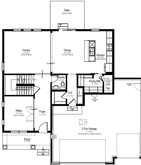
MAIN FLOOR - 3 CAR GARAGE (28')
