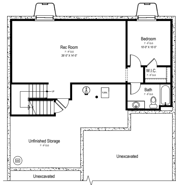
OPT. FINISHED BASEMENT PARTIAL BASEMENT FLOOR PLAN
