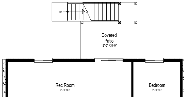
OPT WALKOUT BASEMENT PARTIAL BASEMENT PLAN
