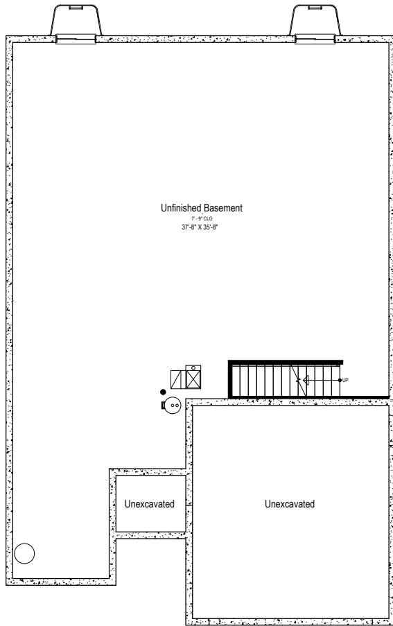
BASEMENT
