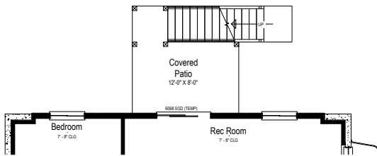
OPT WALKOUT BASEMENT PARTIAL BASEMENT FLOOR PLAN
