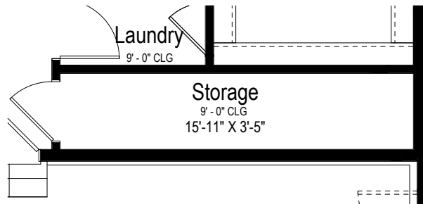
Crawl Space Storage Partial Main Floor Plan
