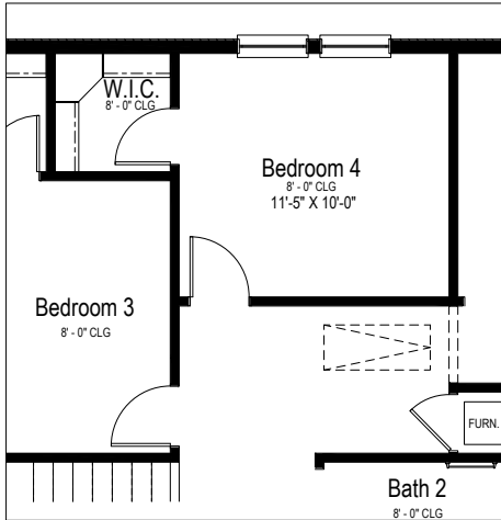
Opt. Bedroom 4 Partial Upper Floor Plan
