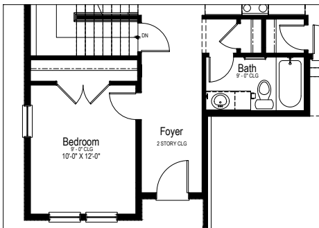
Opt. Bedroom w/ Bath Partial Main Floor Plan
