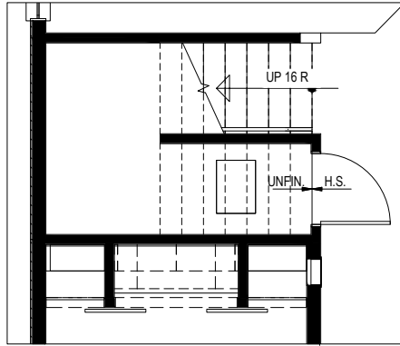
Opt. Crawl Space Partial Main Floor Plan
