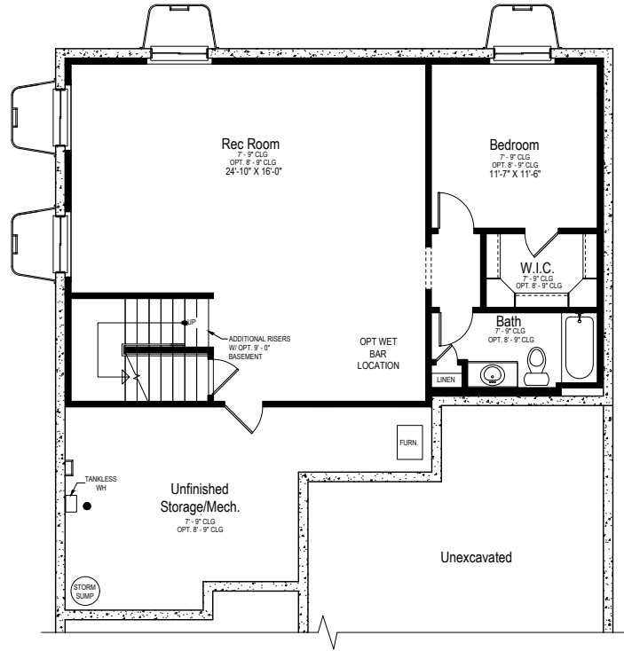
OPT. FINISHED BASEMENT PARTIAL BASEMENT FLOOR PLAN
