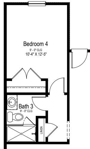
Partial Main Floor Plan Opt. Bedroom 4
