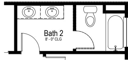
Opt. Alt. Bath 2 Partial Upper Floor Plan
