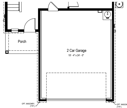
Opt. 4' Garage Extension Partial Main Floor Plan
