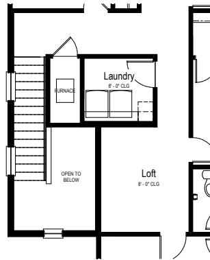
Opt Loft/Laundry Partial Upper Floor Plan
