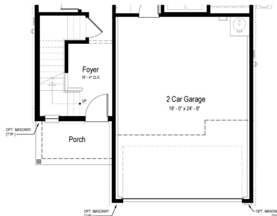
Opt. 4'-0" Garage Extension Partial Main Floor Plan
