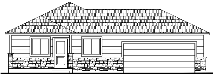
FOOTHILLS ELEVATION - OPT 2 CAR GARAGE
