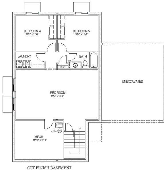
OPT FINISH BASEMENT
