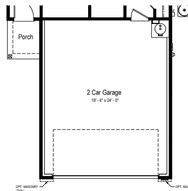
Opt. 4'-0" Garage Extension Partial Main Floor Plan
