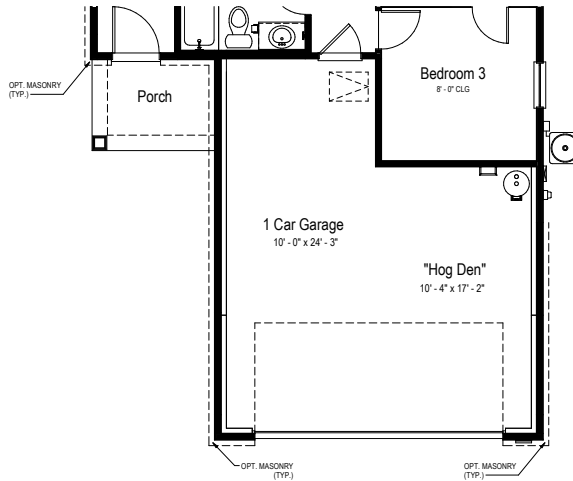
Opt. 4' Garage Extension Partial Main Floor Plan
