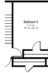
Opt Bedroom 5 Partial Upper Floor Plan
