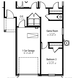
Opt. Game Room Partial Main Floor Plan
