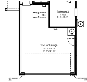
Opt. 4'-0" Garage Extension Partial Main Floor Plan
