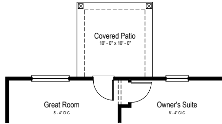
Opt. Covered Patio Partial Main Floor Plan
