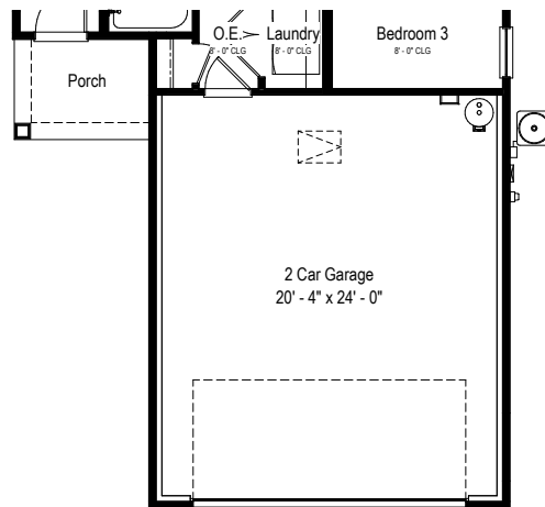
Opt. 4' Garage Extension Partial Main Floor Plan
