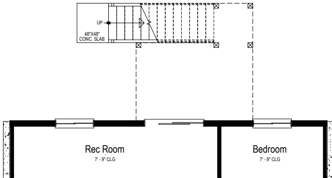
OPT WALKOUT BASEMENT PARTIAL BASEMENT PLAN
