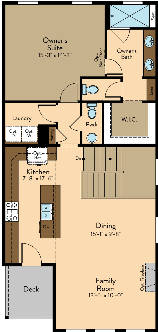
Upper Level Floor Plan
