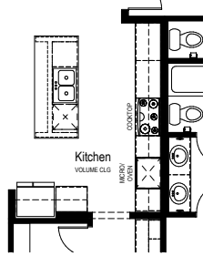
Opt. Gourmet Kitchen Partial Main Floor Plan
