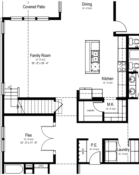
Opt. Bonus Room Partial Main Floor Plan
