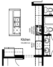
Opt. Chef Kitchen Partial Main Floor Plan
