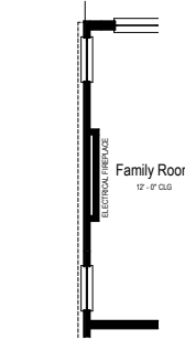
Opt. Fireplace Family Room Partial Main Floor Plan
