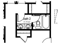
Opt. Bath 2 Double Sink Partial Main Floor Plan
