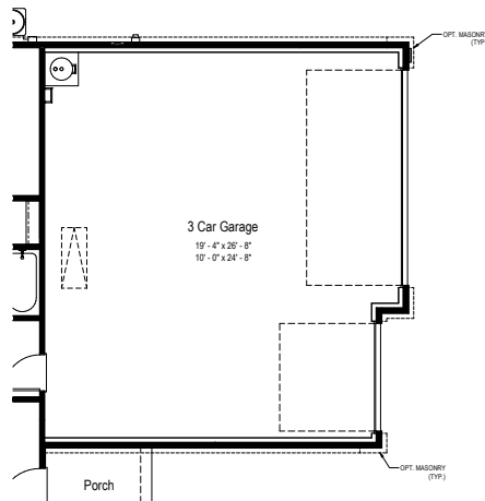
Opt. 4'-0" Garage Extension Partial Main Floor Plan
