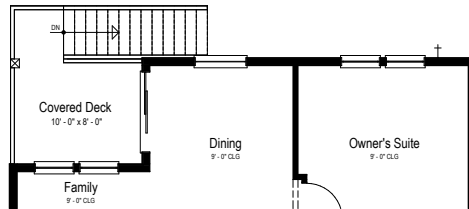
Opt. Daylight Basement Partial Main Floor Plan
