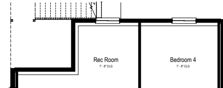
Opt. Daylight Basement Partial Basement Plan
