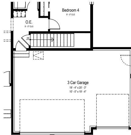
Partial Main Floor Plan
