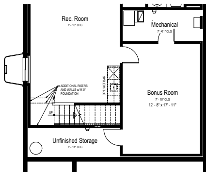
Opt. Bonus Room Partial Finished Basement Plan
