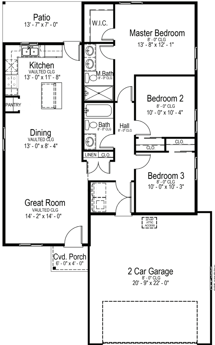
SHERIDAN - FLOOR PLAN
